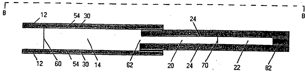
Cross Section Along Line B-B' of FIG. 4
